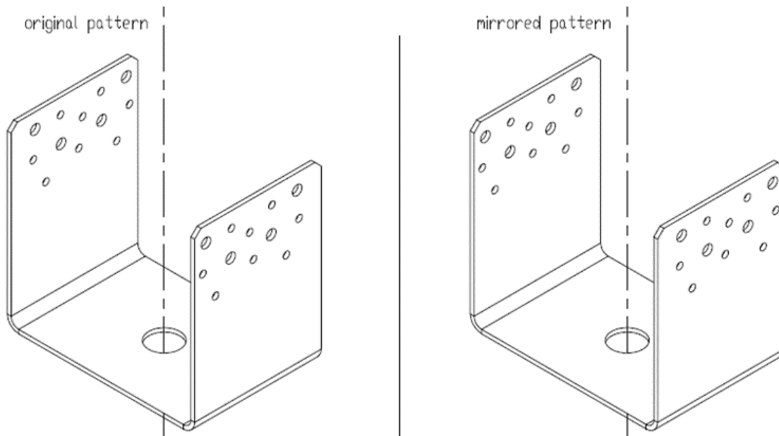
Figure 5. U-Plate Top Plate Variants
