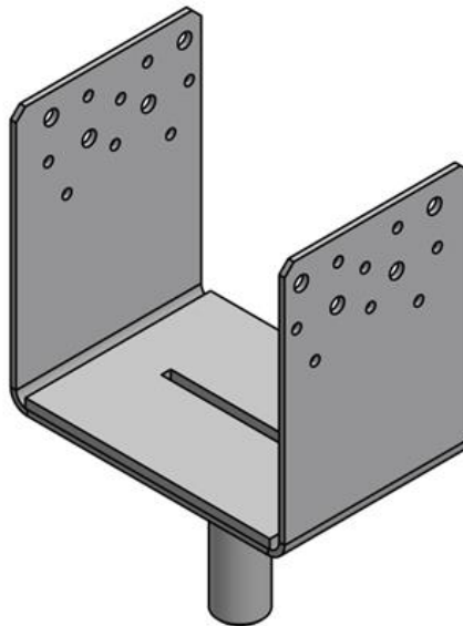
Figure 4. Completed U-Plate Top Plate
