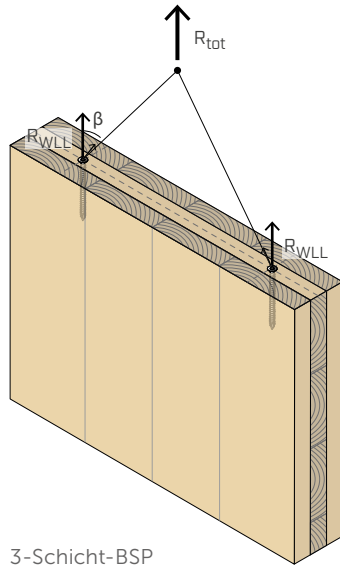
3-Schicht-BSP
