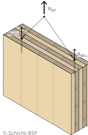
5-Schicht-BSP
