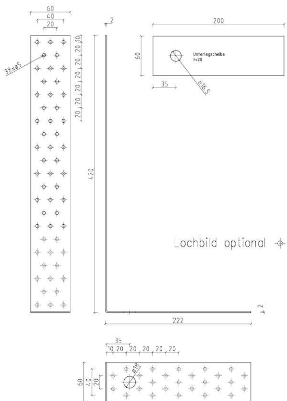
Figure B. 9 Dimensions of type WZU422
