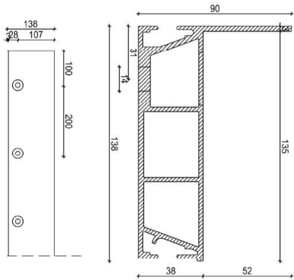
Figure C.6: ALU START 120 – Longitudinal section and top view
